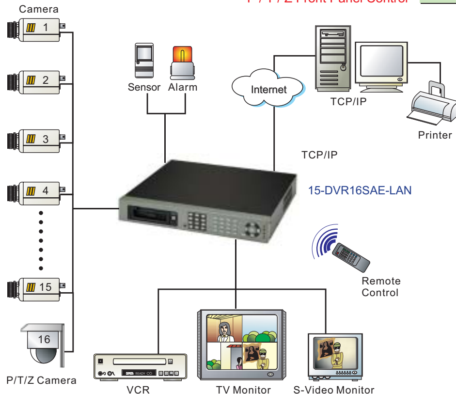
P / T / Z Front Panel Control 15-DVR16SAE-LAN
